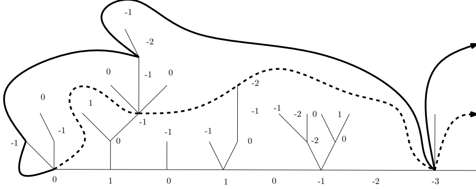
FIGURE 3.5. The maximal (in solid line) and minimal (in dotted line) geodesics starting from the root corner of the tree \theta .
