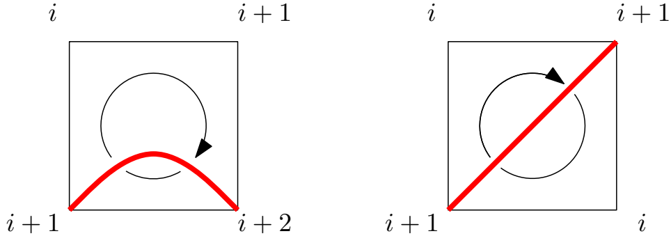
FIGURE 2.2. Rules for the reverse Schaeffer construction.
