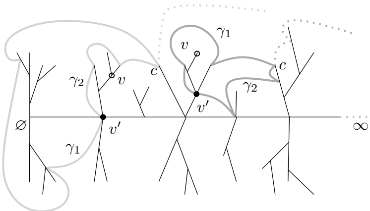
FIGURE 5.11. Cycles separating vertices from \emptyset composed by two geodesics.
