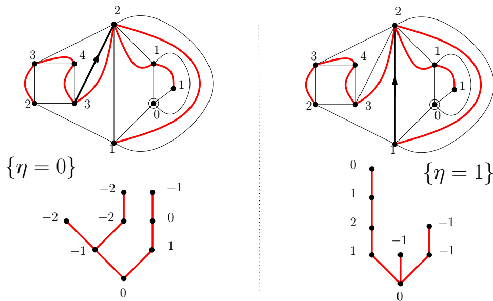
FIGURE 2.3. Illustration of the rooting of the plane tree \tau
