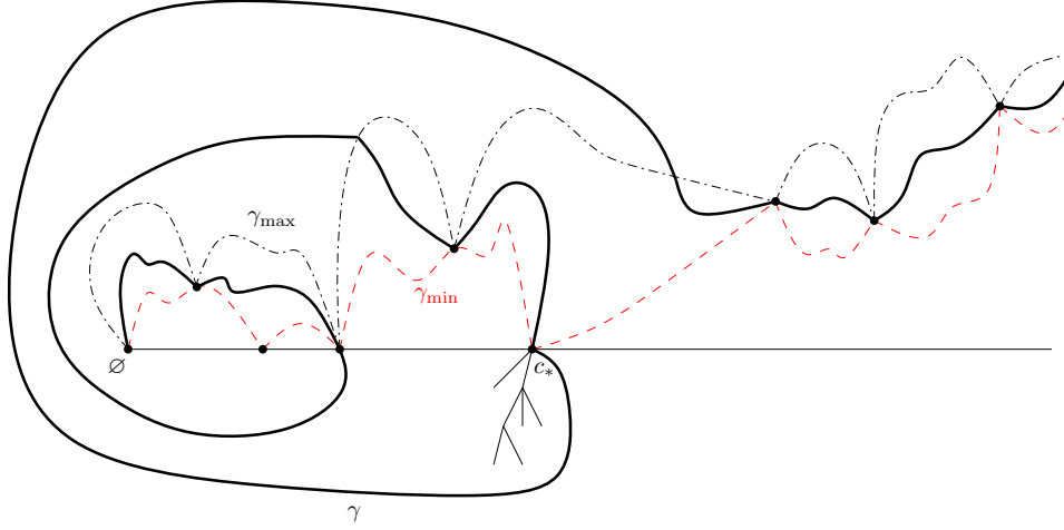
FIGURE 3.8. Illustration of the proof of Theorem 3.4: A proper geodesic can “swirl” around T_\infty by traversing the spine, but is eventually trapped between the minimal and maximal geodesics
