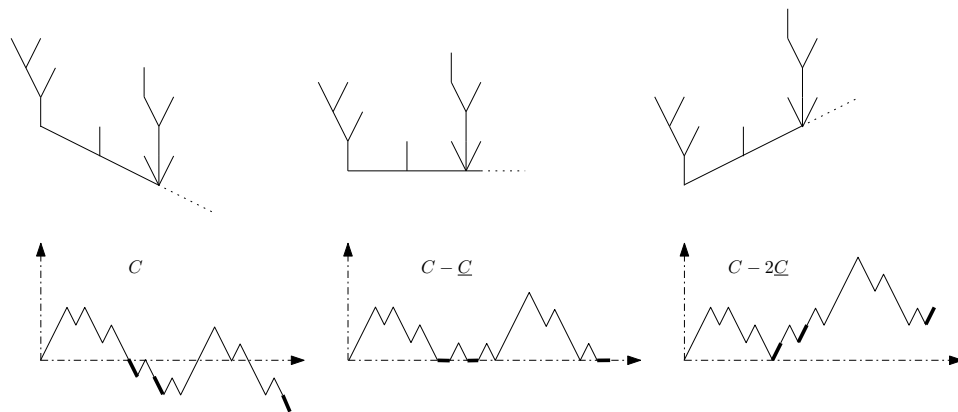
FIGURE 4.10. Different codings of a forest
