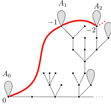
FIGURE 3.7. The second step of the exploration.
