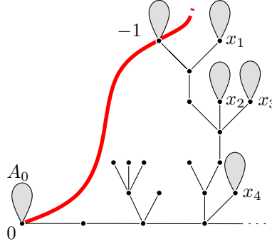
FIGURE 3.6. Exploration of T_\infty until the first -1 . The gray trees are unexplored.
