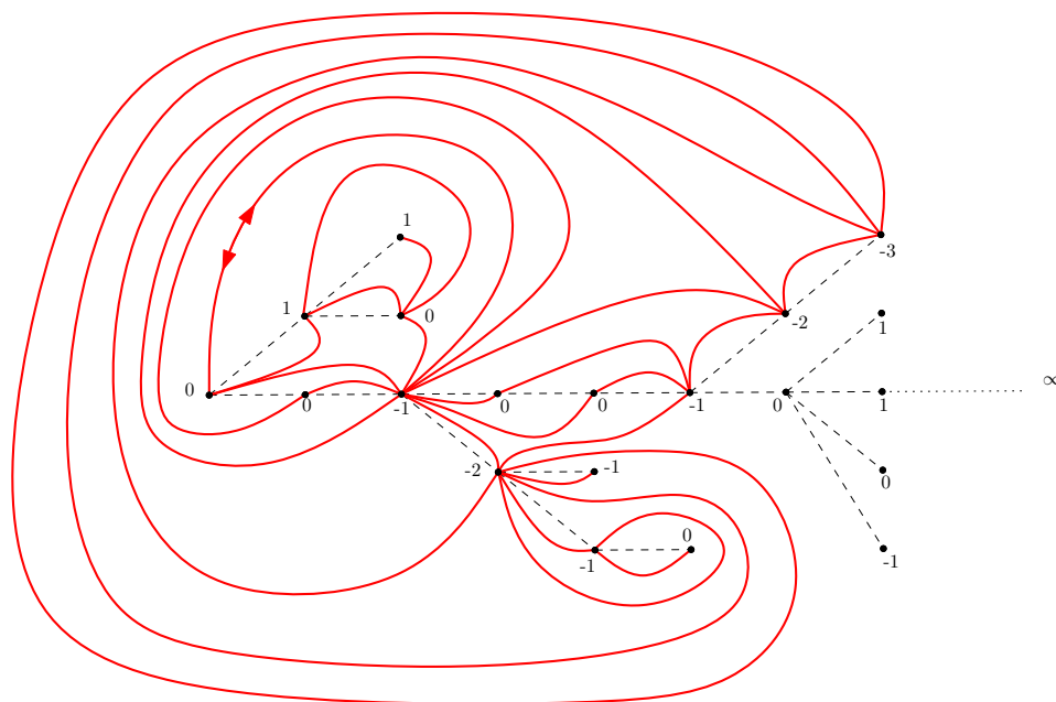
FIGURE 2.1. Illustration of the Schaeffer correspondence. The tree is represented in dotted lines and the quadrangulation in solid lines.
