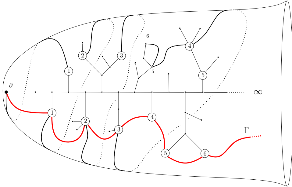
FIGURE 3.4. Illustration of the proof of Lemma 3.3. The tree is represented in solid lines. Every vertex marked by a circled integer corresponds to the last occurrence of this integer along either the left or the right side of the tree. The distinguished geodesic \Gamma is represented by a thick line.
