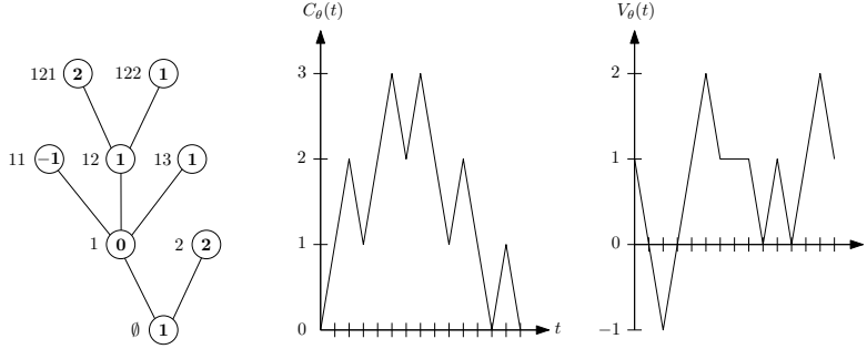
FIGURE 4.9. A labeled tree \theta and its pair of contour functions (C_\theta, V_\theta) .
