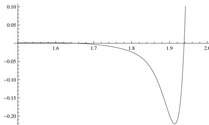
FIGURE 4.17. \det((K'_{2i+2j-2})_{i,j=1}^4) as a function of r .
