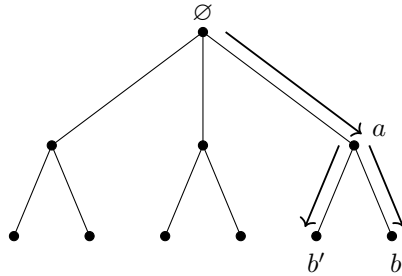
FIGURE 2.7. A representation of D_1 , defined as the event in which the frog coming from the root and the frog at the first vertex it hits (labelled a in the figure above) go to different children of a .
