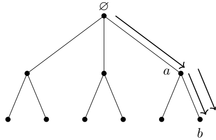
FIGURE 2.2. A depiction of a scenario in which a node on an even level (node b ) has two frogs land on it from above simultaneously without being stopped. Note that in order for such an event to accord with the specifications of the self-similar model, the two frogs landing on b must be the frog originating at the parent node of b (labeled a in the figure) and the frog that activated the frog at the parent of b .
