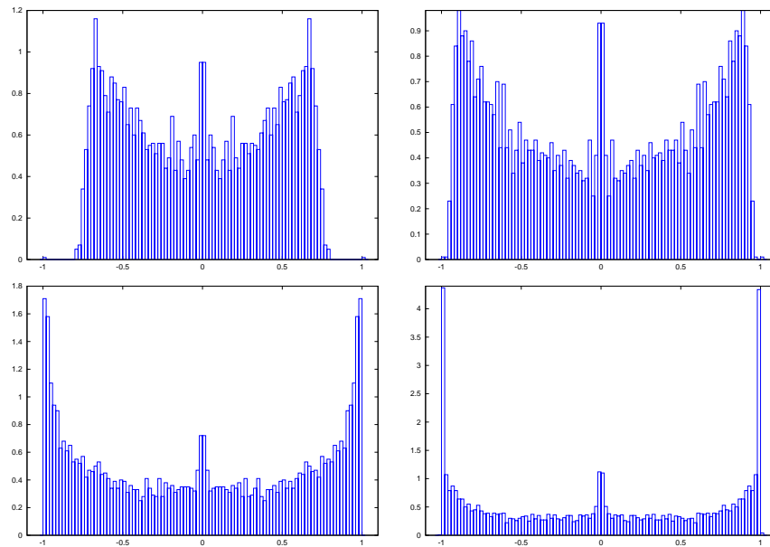
FIGURE 3.2. Plots illustrating Corollary 1.7 and the second statement of Theorem 1.10. Each histogram corresponds to the spectrum of a single realization of K with n = 5000 , for various choices of \mathcal{L} . From left to right and top to bottom, \mathcal{L} is uniform on [0, t] with t = 1/8, t = 1/4, t = 1/2 , and t = 1 .
