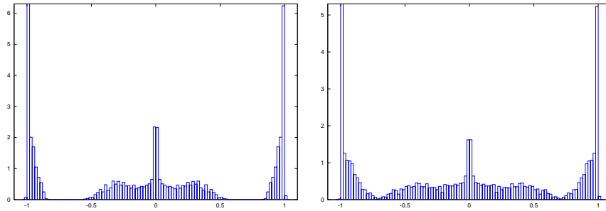
FIGURE 3.1. Plots illustrating Corollary 1.7. Each histogram corresponds to the spectrum of a single realization of K with n = 5000 , for various choices of \mathcal{L} . From left to right \mathcal{L} is the uniform law on [0, t] \cup [1 - t, 1] for t = 1/8, t = 1/4 .
