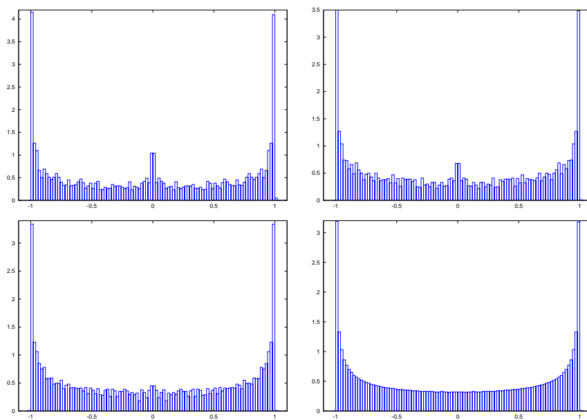
FIGURE 3.3. Plots illustrating Corollary 1.7. Each histogram corresponds to the spectrum of a single realization of K with n = 5000 , for various choices of \mathcal{L} . From left to right and top to bottom, \mathcal{L} is uniform on [t, 1 - t] with t = 0 , t = 1/8 , t = 1/4 , t = 1/2 . The last case corresponds to the arc-sine limiting spectral distribution mentioned in Remark 1.8.
