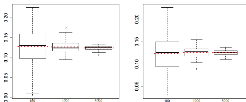
FIGURE 2.2. Box plots of the approximations of E(V|U = 0.5) as a function of the number of simulations, m , for \epsilon = 0.1 and \epsilon = 0.01 .
