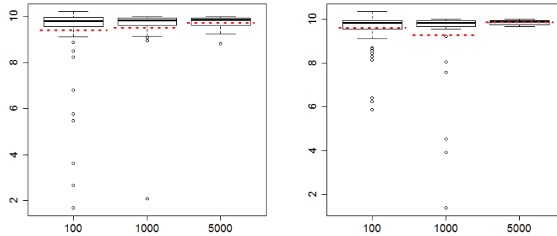
FIGURE 3.3. Box plots of the approximations of \xi^{\circ} & MSE as a function of the number of simulations, m , for \epsilon = 0.1 and \epsilon = 0.01 .
