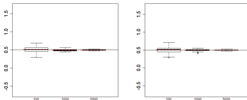
FIGURE 2.1. . Box plots of the approximations of E(Y|X = 1) as a function of the number of simulations, m , for \epsilon = 0.1 and \epsilon = 0.01 .
