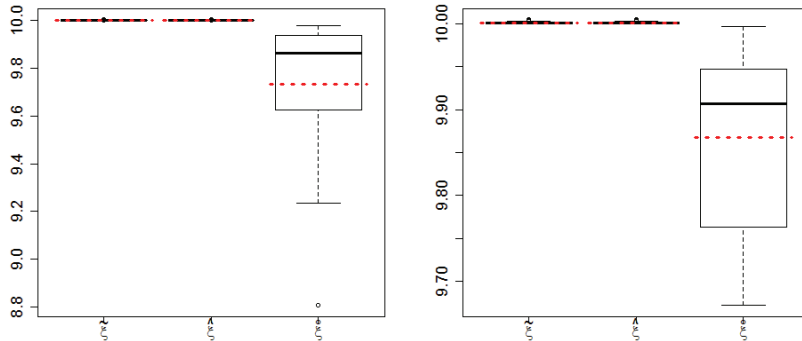
FIGURE 3.4. Box plots of the approximations of \xi , \hat{\xi} and \tilde{\xi} as a function of the number of simulations, m = 100, 1000, 5000 , for \epsilon = 0.1 and \epsilon = 0.01 .
