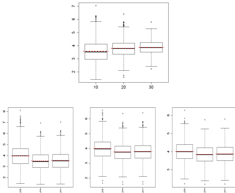
FIGURE 4.5. Box plots for the estimator \hat{\eta} for sample sizes n = 10, 20, 30 (above) and for the estimators \tilde{\eta} , \hat{\eta} y \hat{\eta} for sample sizes n = 10, 20, 30 , respectively (below).
