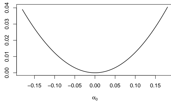
FIGURE 2.2. Graph of the function F(\alpha_0) = I(\hat{x}_{\alpha_0}) , that is, a parametric version of the rate function.
